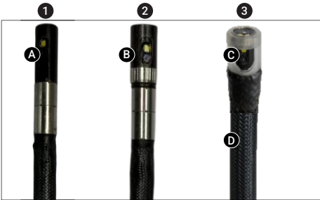
1 6.0mm Standard probe 2 Optional: Probe with protective cap 7 & 10 meters 3 Optional: Plastic sleeve probe for 7 & 10 meters
